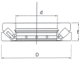
Thrust Spherical
