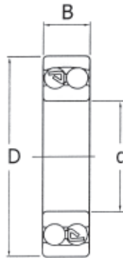
Cylindrical bore
