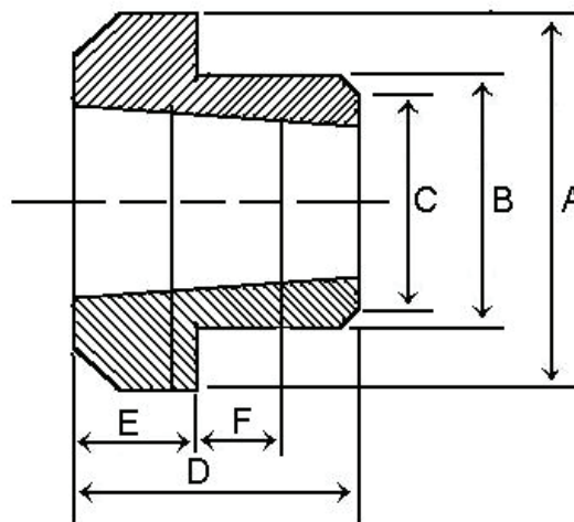
WH Weld on hubs
