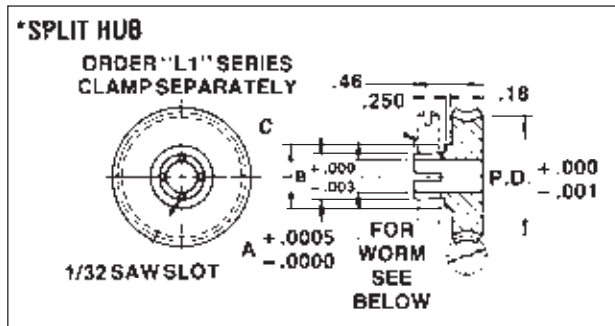
SPLIT HUB
