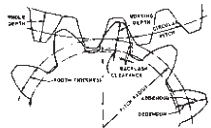
FIGURE 2.2 — SPUR, HELICAL, GEAR NOMENCLATURE
