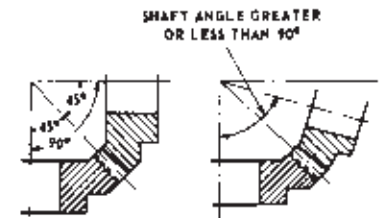
FIGURE 1.5b — MITER GEARS
