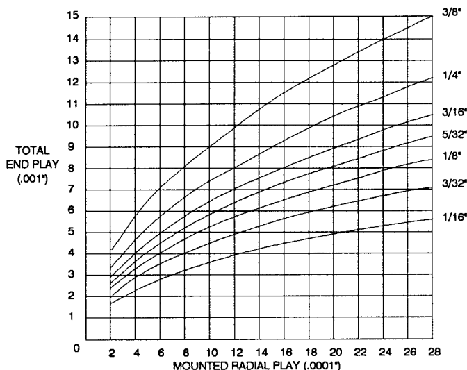
Figure 7: End Play vs. Radial Play
