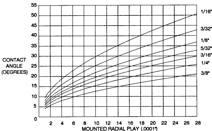
Figure 6: Contact Angle vs. Radial Play
